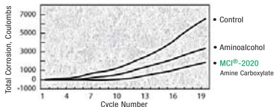
Cracked Beam Testing of Surface Treatments. Details: www.CortecMCI.com
