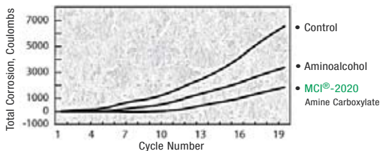
Cracked Beam Testing of Surface Treatments. Details: www.CortecMCI.com
